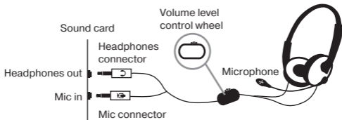
Fig. 1. Connection diagram
