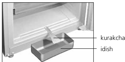
7 rasm — MBdan erigan suvni yig'ib olish
