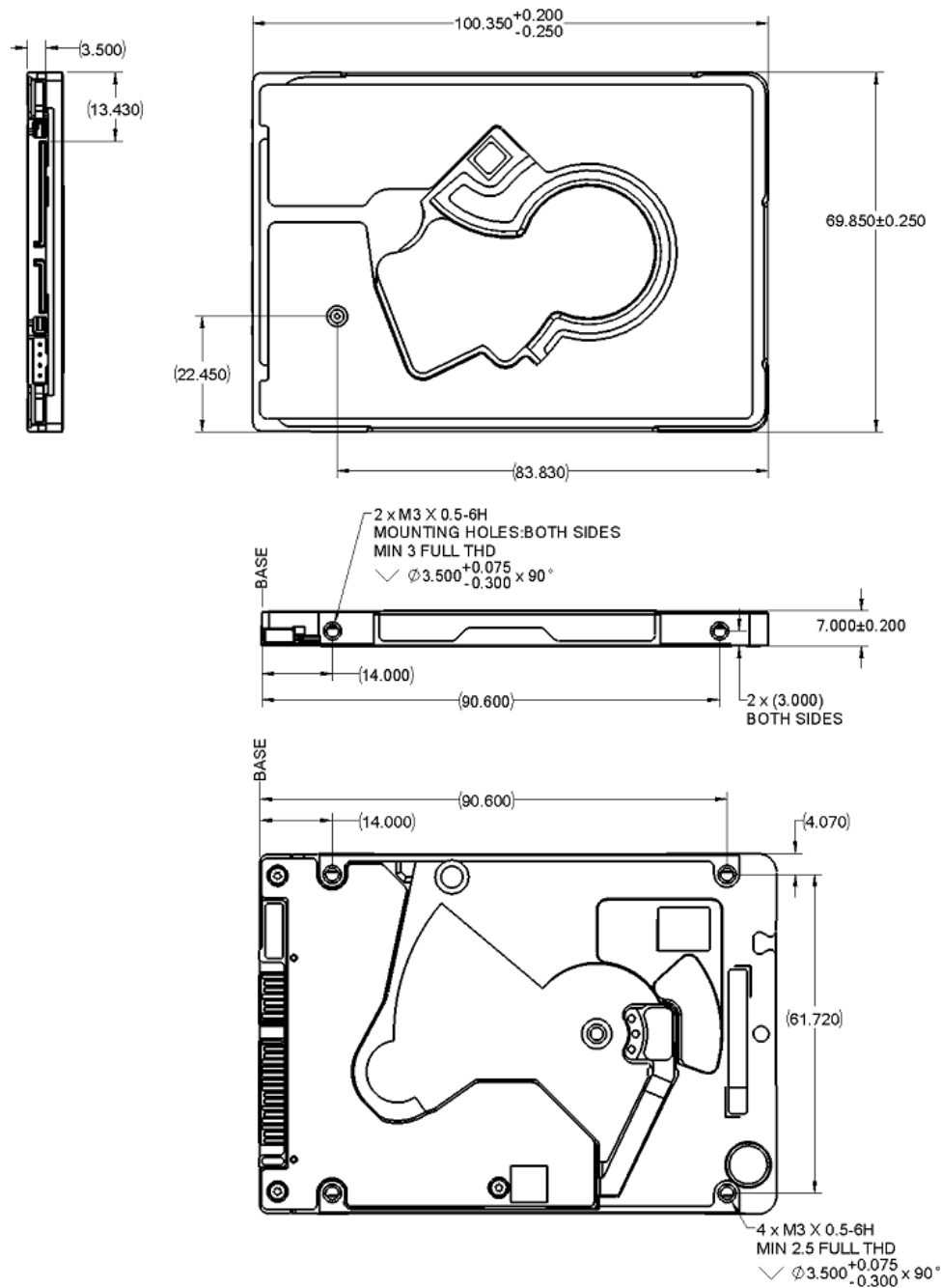
Figure 4 Mounting Dimensions
