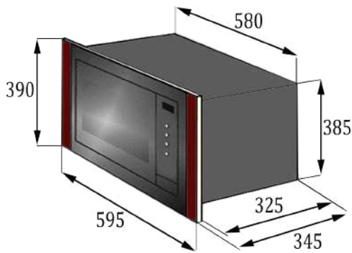
EOK 28 X
