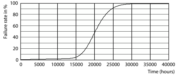
Life Expectancy Diagram - DN020B G3 LED20/NW 23W 220-240V D200 GM
