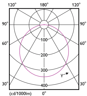
Light Distribution Diagram - DN020B G3 LED20/NW 23W 220-240V D200 GM
