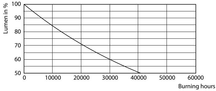
Lumen Maintenance Diagram - DN020B G3 LED20/NW 23W 220-240V D200 GM
